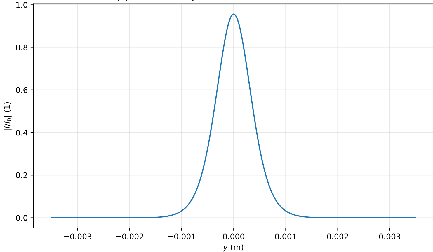
Intensity profile I(x=0, y, z=1.513)/I_0 , \text{Pin}=0.5\text{Pcr} , artificial time
